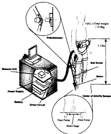
Fig.2.2 HAL system
