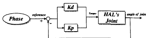
Fig.2.5 Joint control system
